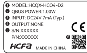
Figure 1 Model name and nameplate description
