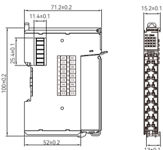
Figure 4 Installation dimension for HCQX-HC04-D2 (unit: mm)
