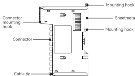
Figure 3 Interface diagram from right view for HCQX-HC04-D2
