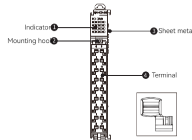
Figure 2 Interface diagram for HCQX-HC04-D2
